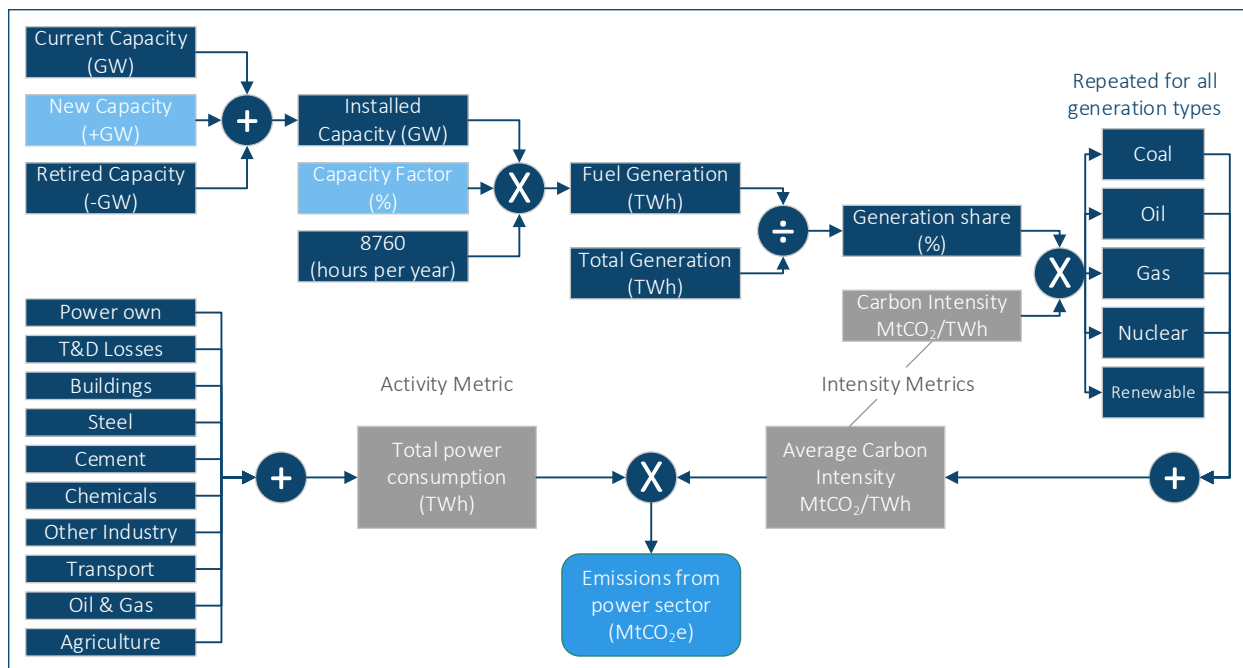
Figure 2: Power Sector Emissions Logic Tree. The CTI model calculates emissions from the power sector based on factors that include activity metrics and intensity metrics (indicated in grey) accounting for various fuel types and energy demand from the sectors (dark blue) as well as the generation necessary to cover own power consumption and transmission and distribution losses. Data are based on BNEF, IEA, and CTI’s own demand forecast from the various other sectors. Light blue indicates where optimization takes effect.
